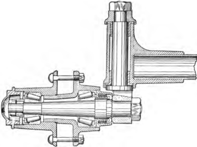
FIG. 461.—Stud Steering Axle showing Hub hung on Conical Roller Bearings. The shape of the bearings serves the double purpose of securing perfect rotative movement in forward travel; also to take up end thrusts.
